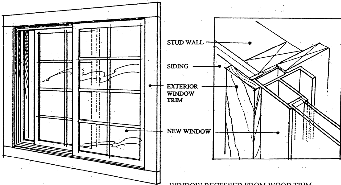
ACCEPTABLE INSTALLATION
