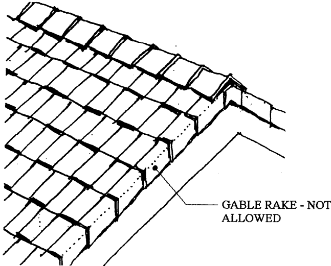
UNACCEPTABLE METHOD
