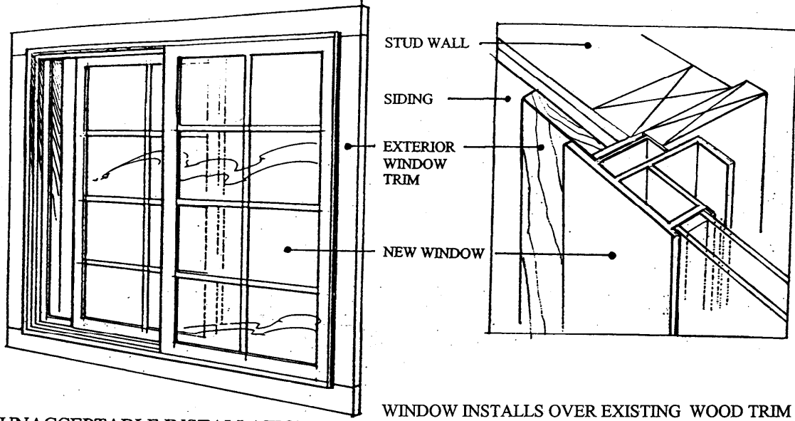
UNACCEPTABLE INSTALLATION
