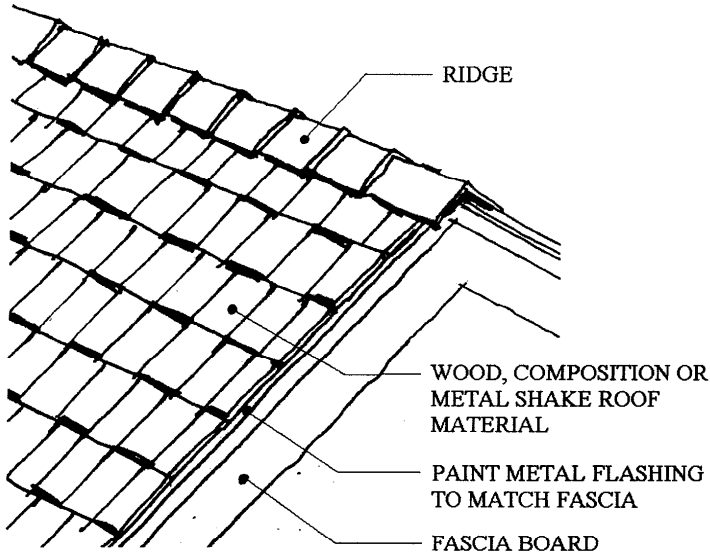
ACCEPTABLE METHOD
